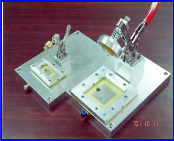
LEAK CHECK JIG
